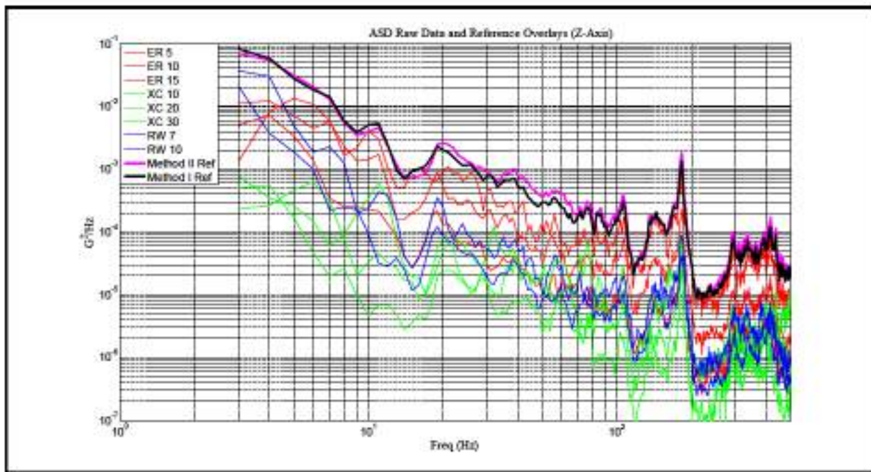
Figure 8. ASD references for the Z axis.
