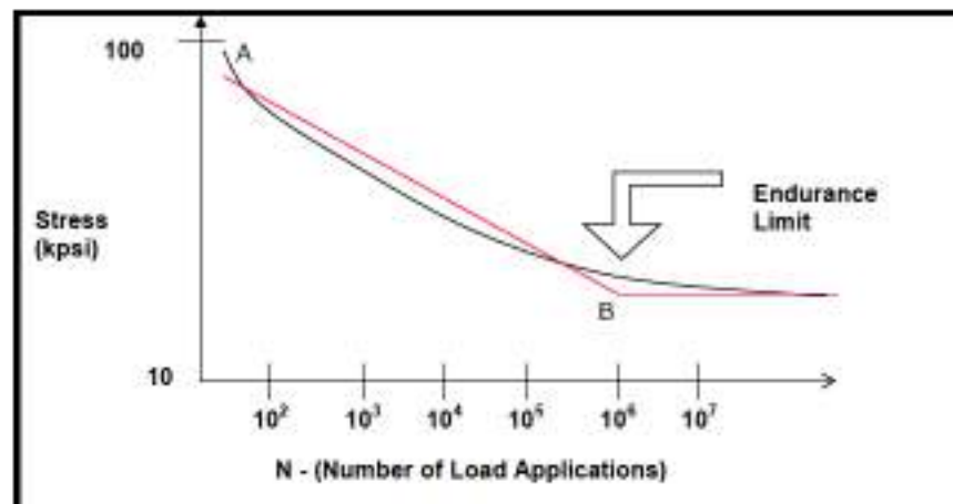
Figure 514.8F-2. S/N curve.
