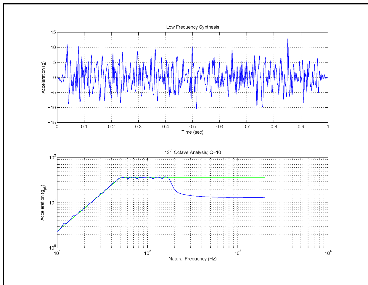
Figure 519.8B-4. Bandlimited random synthesis (10 Hz – 200 Hz).
