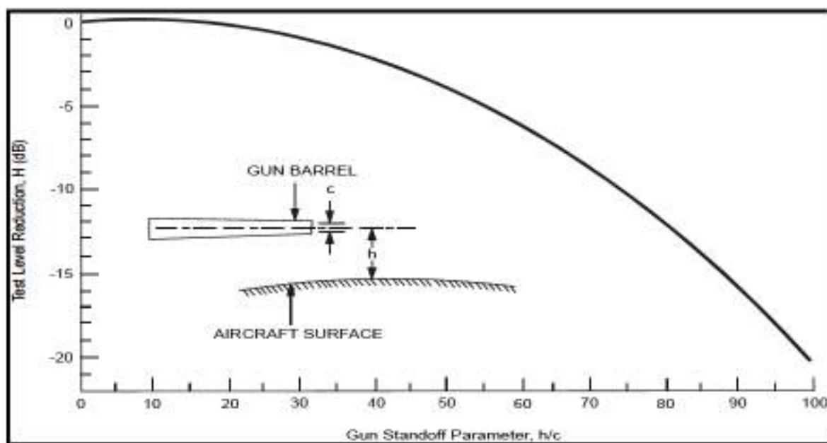
Figure 519.8C-4. Test level reduction due to gun standoff parameter.
