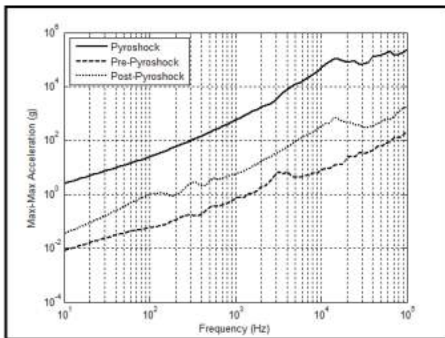
Figure 517.3-5. Acceleration maximax SRS for the pyroshock, pre-pyroshock and post pyroshock (laser).
