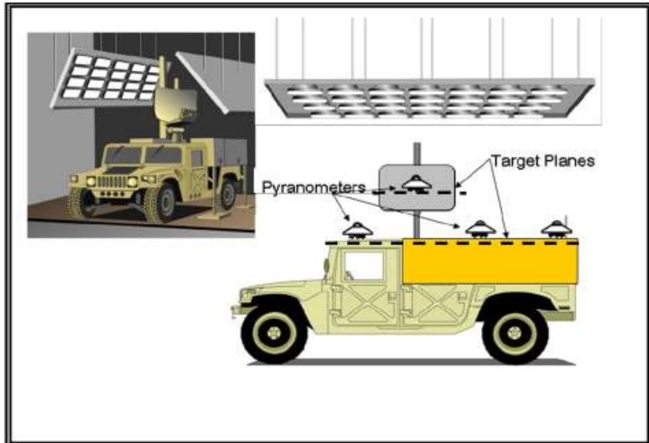
Figure 505.7C-4. Example 3 - Multiple solar surface target planes.
