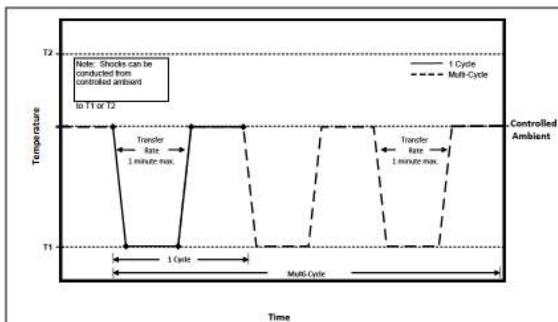
Figure 503.7-4. Shocks to &amp; from Controlled Ambient.
