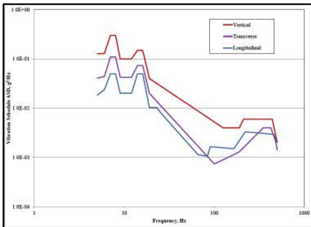
Figure 514.8C-6. – Category 4 – Composite wheeled vehicle vibration exposure.
